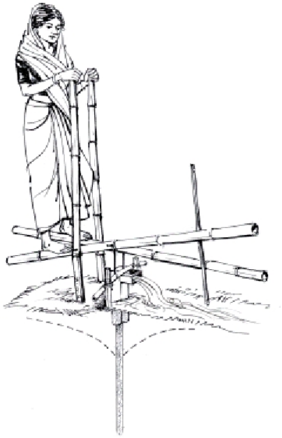
Figure 4. Woman operating a basic treadle pump (with a bamboo support structure and treads and metal cylinders and pistons) that is supplied from a borehole.
